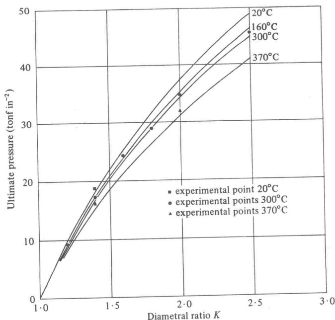
Figure 22. Ultimate pressure of Vibrac cylinders calculated from torsion data.
