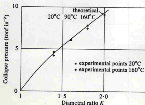
Figure 24. Collapse pressure of EN3A cylinders at 20 and 160 ^{\circ}\text{C} .
