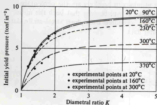
Figure 23. Initial yield pressure of EN3A cylinders at various temperatures.
